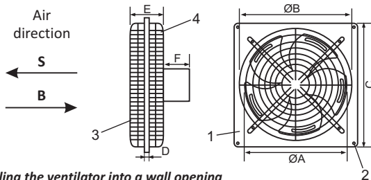
FIG. 1 - Installing the ventilator into a wall opening
